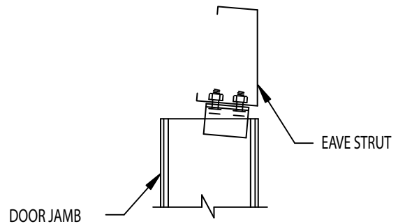
JAMB TO EAVE STRUT
