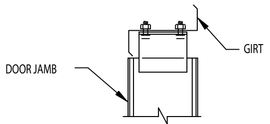
JAMB TO GIRT
