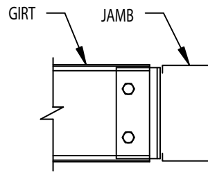
GIRT TO JAMB CONN.
