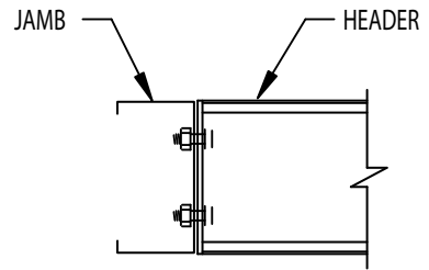
HEADER TO JAMB CONN.
